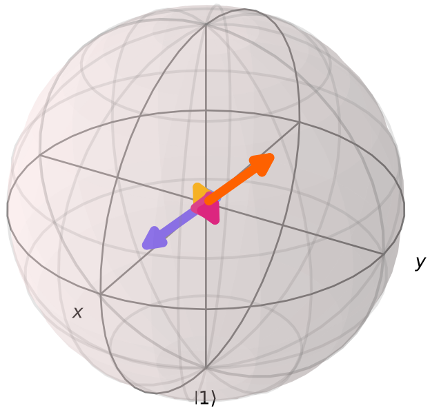
qubit 0 |0\rangle
