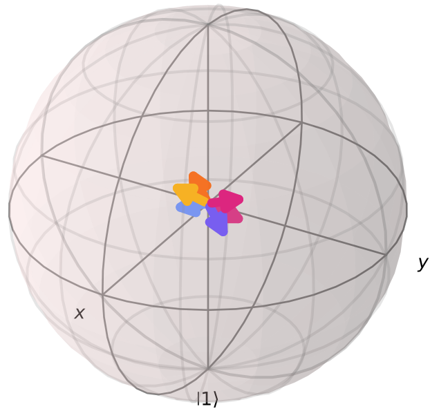
qubit 1 |0\rangle
